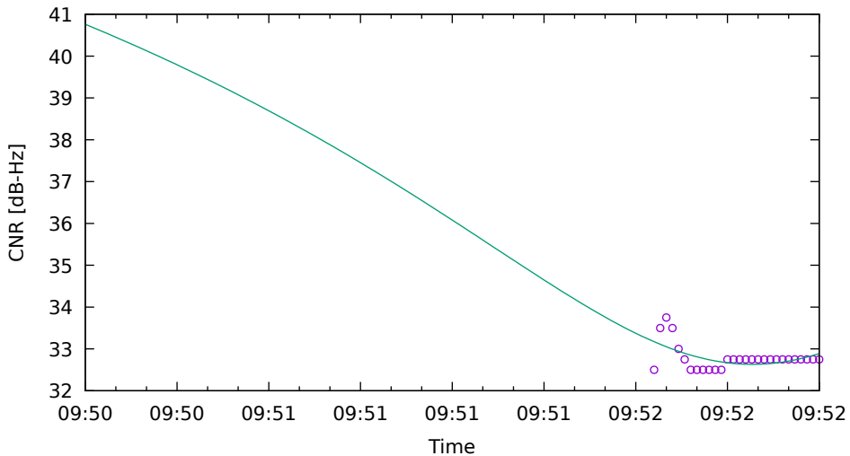
CNR fit for E36 on Xiaomi11T - drive 18 (DOY262)
