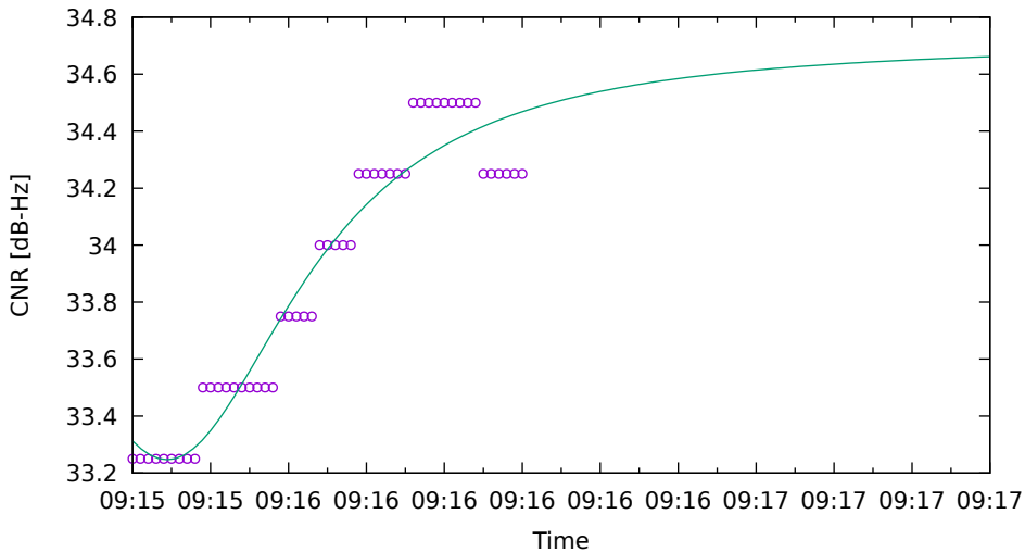
CNR fit for G01 on Xiaomi11T - drive 1 (DOY262)
