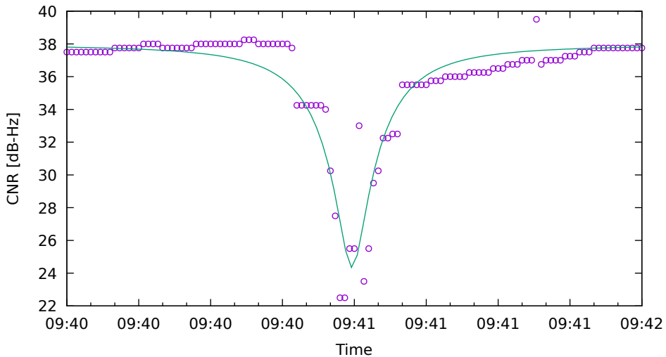
CNR fit for G01 on Xiaomi11T - drive 13 (DOY262)
