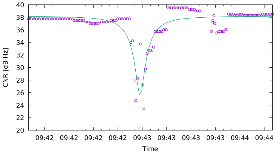
CNR fit for G01 on Xiaomi11T - drive 14 (DOY262)
