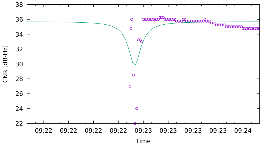
CNR fit for G01 on Xiaomi11T - drive 4 (DOY262)
