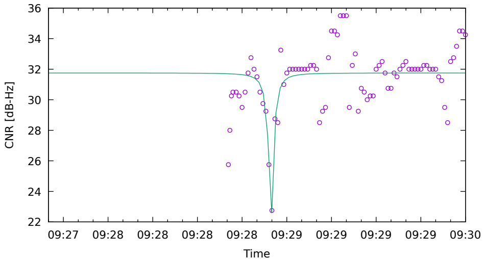
CNR fit for G01 on Xiaomi11T - drive 7 (DOY262)
