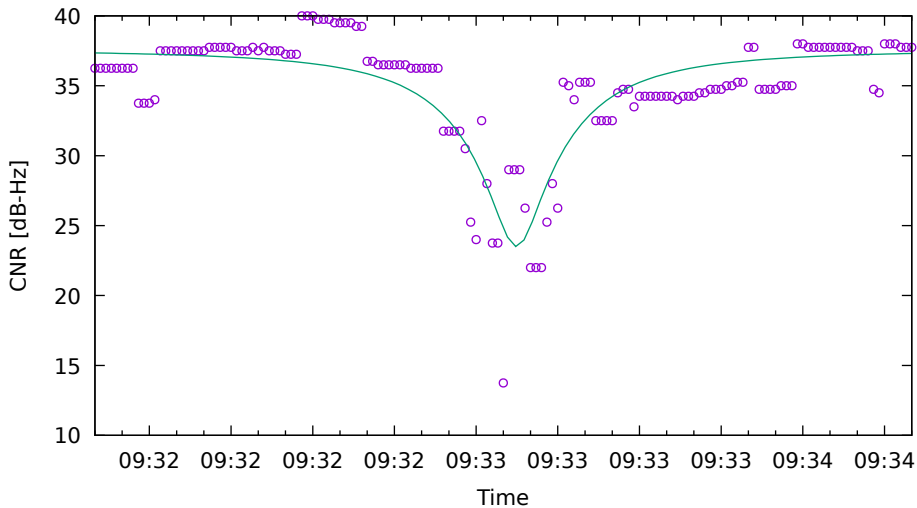
CNR fit for G01 on Xiaomi11T - drive 9 (DOY262)
