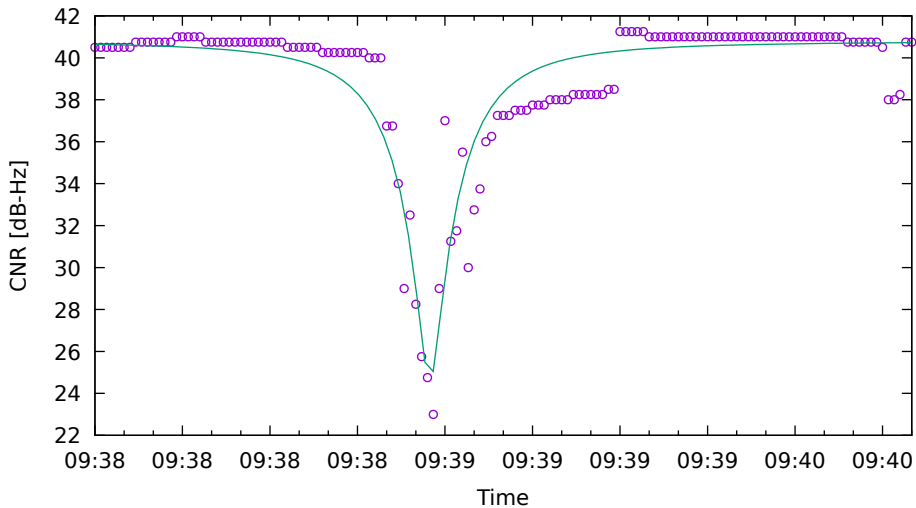
CNR fit for G03 on Xiaomi11T - drive 12 (DOY262)
