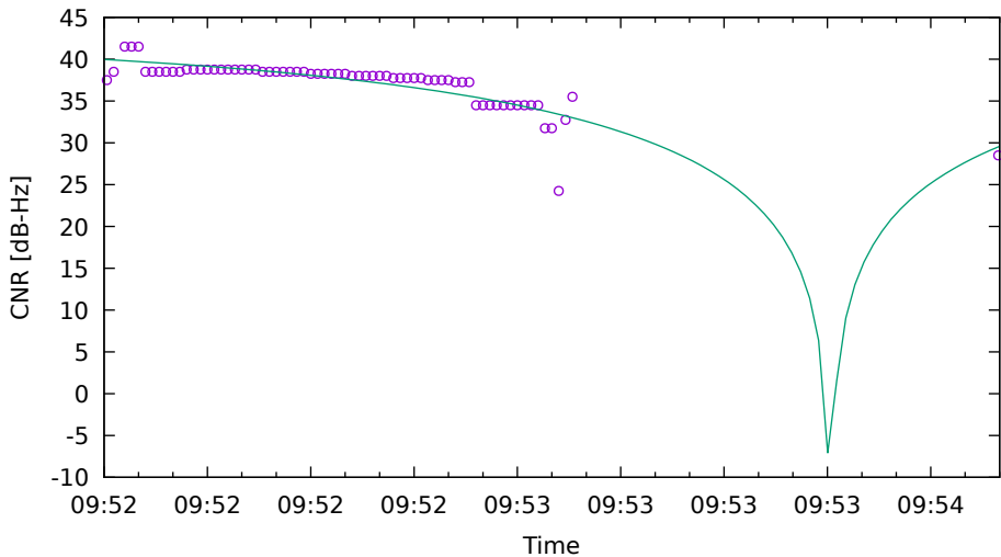
CNR fit for G03 on Xiaomi11T - drive 19 (DOY262)
