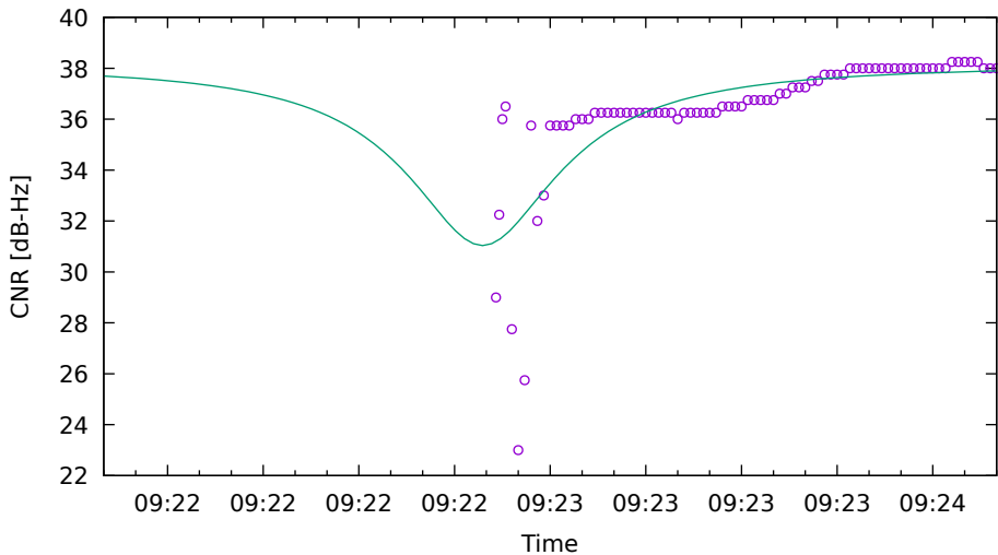
CNR fit for G03 on Xiaomi11T - drive 4 (DOY262)
