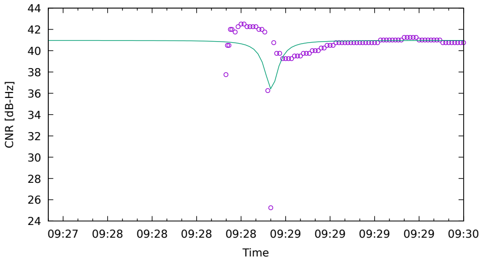
CNR fit for G03 on Xiaomi11T - drive 7 (DOY262)
