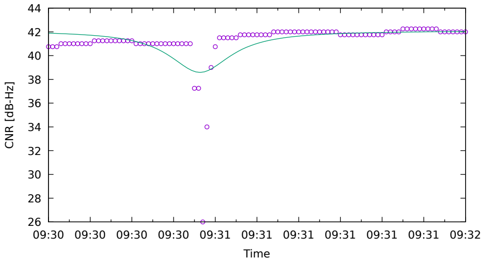
CNR fit for G03 on Xiaomi11T - drive 8 (DOY262)
