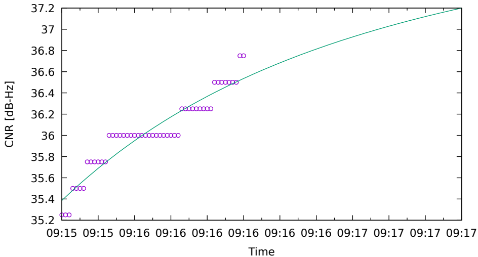
CNR fit for G04 on Xiaomi11T - drive 1 (DOY262)
