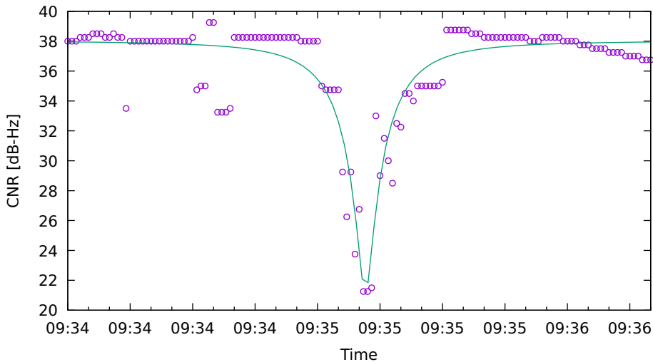
CNR fit for G04 on Xiaomi11T - drive 10 (DOY262)
