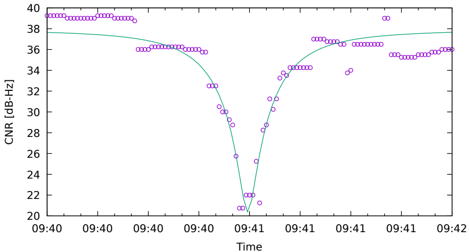
CNR fit for G04 on Xiaomi11T - drive 13 (DOY262)
