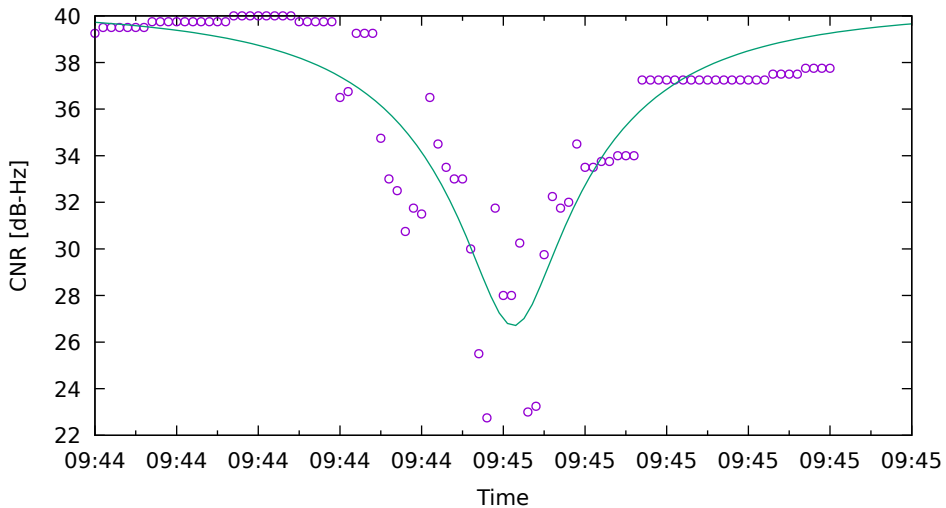
CNR fit for G04 on Xiaomi11T - drive 15 (DOY262)
