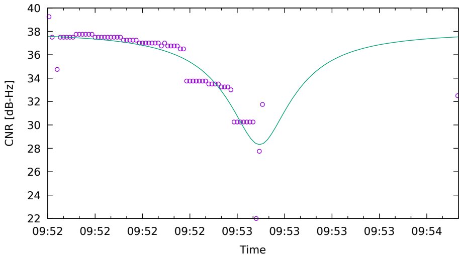
CNR fit for G04 on Xiaomi11T - drive 19 (DOY262)
