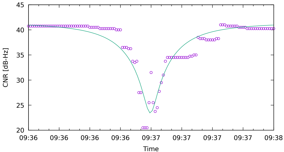
CNR fit for G17 on Xiaomi11T - drive 11 (DOY262)
