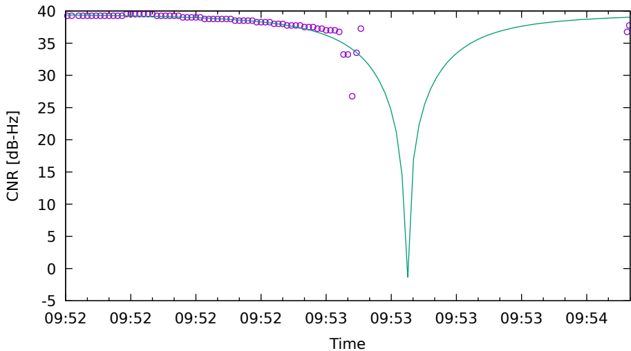
CNR fit for G17 on Xiaomi11T - drive 19 (DOY262)
