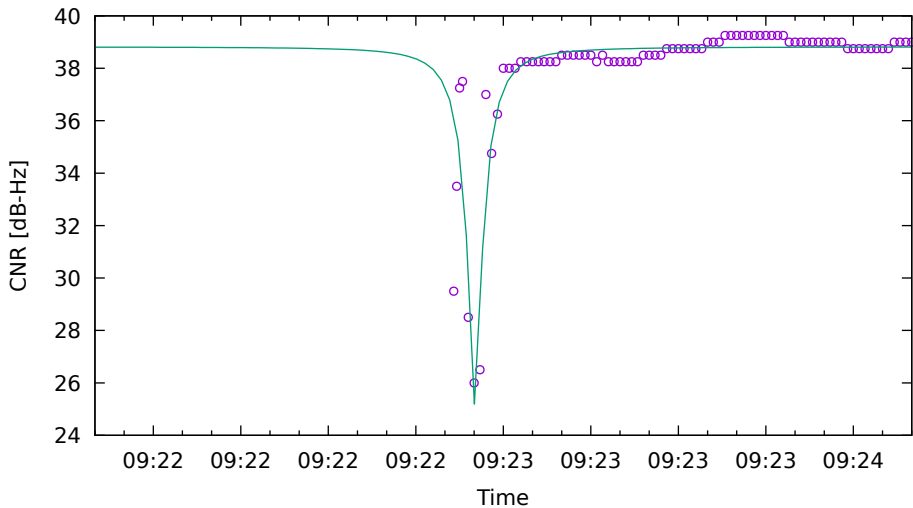
CNR fit for G17 on Xiaomi11T - drive 4 (DOY262)
