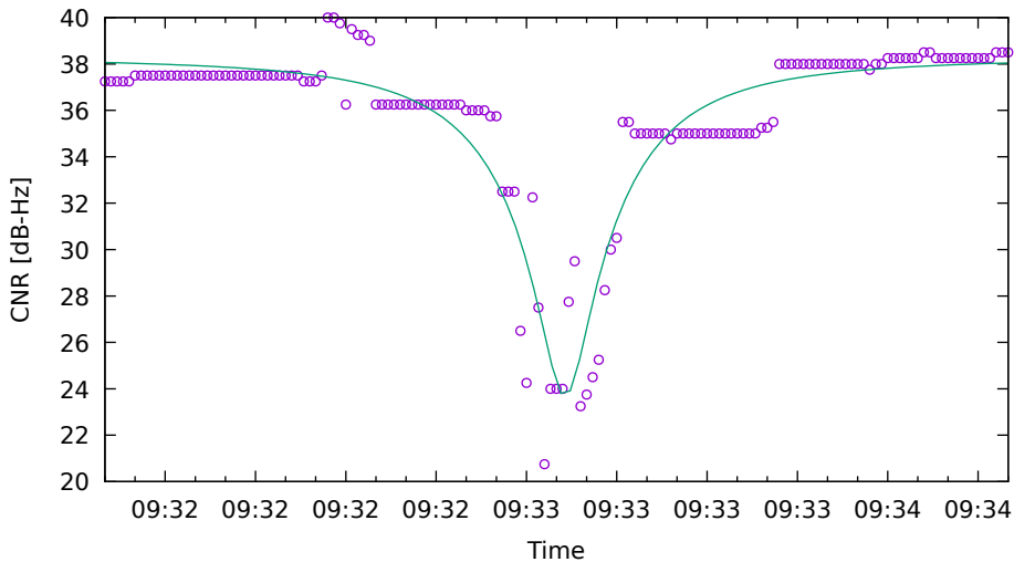
CNR fit for G17 on Xiaomi11T - drive 9 (DOY262)
