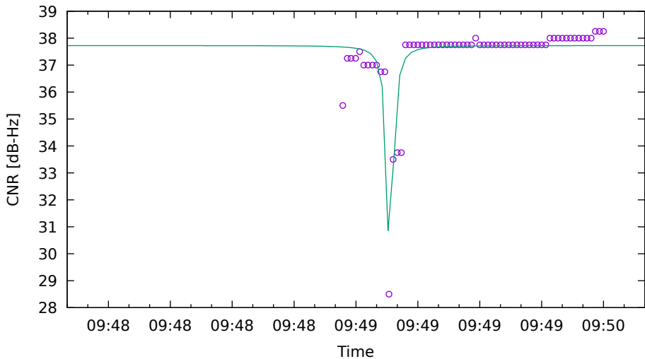
CNR fit for G19 on Xiaomi11T - drive 17 (DOY262)
