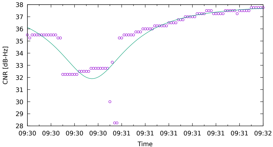
CNR fit for G19 on Xiaomi11T - drive 8 (DOY262)
