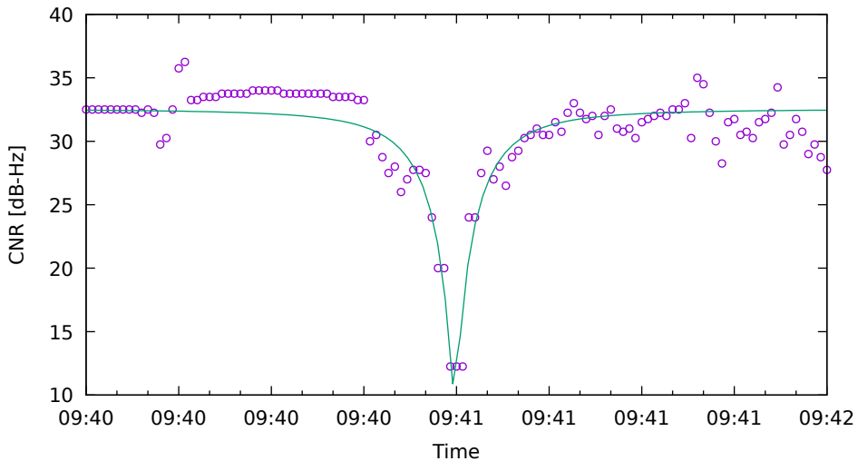
CNR fit for G21 on Xiaomi11T - drive 13 (DOY262)
