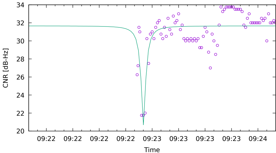
CNR fit for G21 on Xiaomi11T - drive 4 (DOY262)
