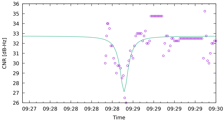
CNR fit for G21 on Xiaomi11T - drive 7 (DOY262)
