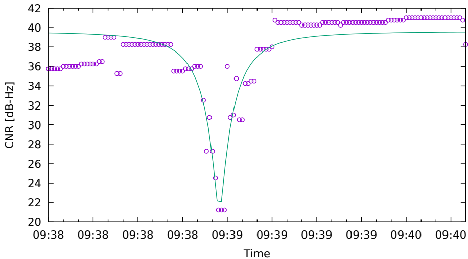
CNR fit for G22 on Xiaomi11T - drive 12 (DOY262)
