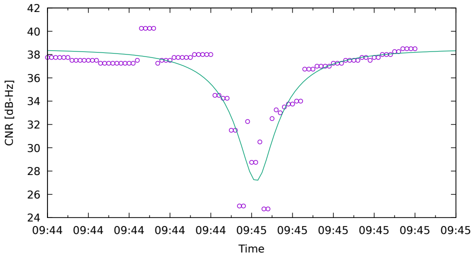
CNR fit for G22 on Xiaomi11T - drive 15 (DOY262)
