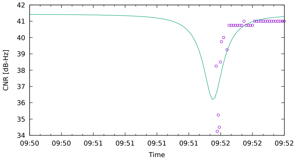
CNR fit for G22 on Xiaomi11T - drive 18 (DOY262)
