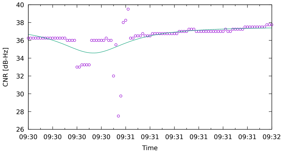
CNR fit for G22 on Xiaomi11T - drive 8 (DOY262)
