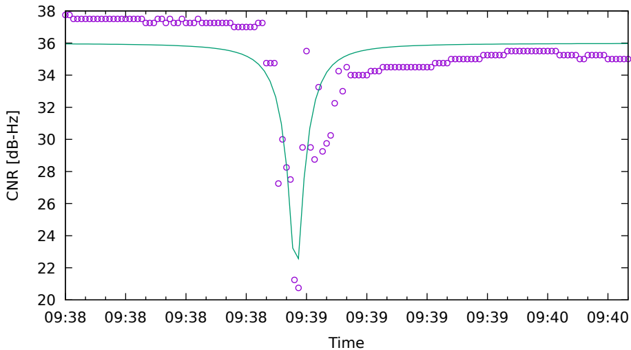
CNR fit for G31 on Xiaomi11T - drive 12 (DOY262)
