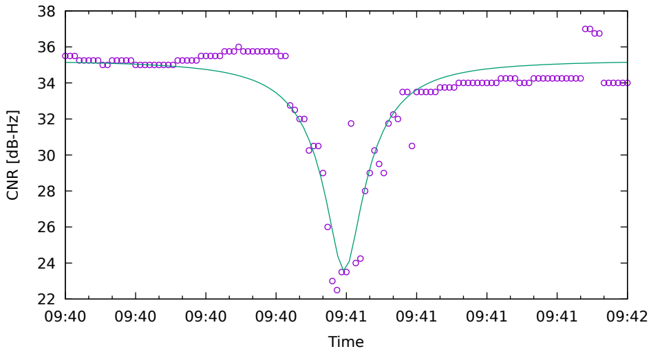
CNR fit for G31 on Xiaomi11T - drive 13 (DOY262)
