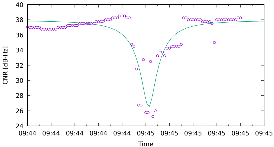
CNR fit for G31 on Xiaomi11T - drive 15 (DOY262)
