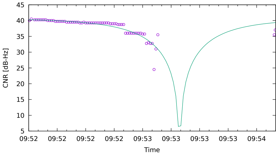
CNR fit for G31 on Xiaomi11T - drive 19 (DOY262)
