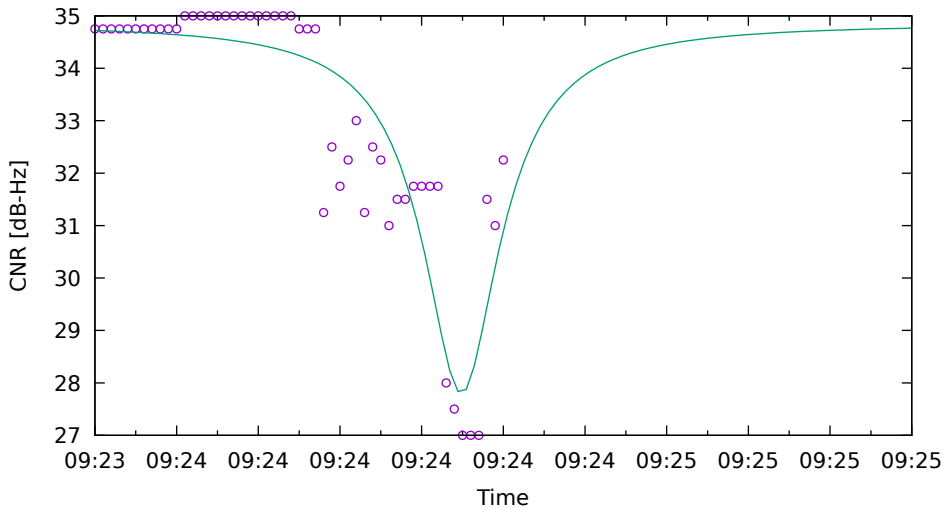
CNR fit for G31 on Xiaomi11T - drive 5 (DOY262)
