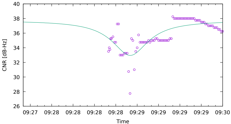
CNR fit for G31 on Xiaomi11T - drive 7 (DOY262)
