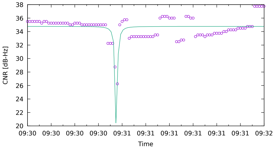
CNR fit for G31 on Xiaomi11T - drive 8 (DOY262)
