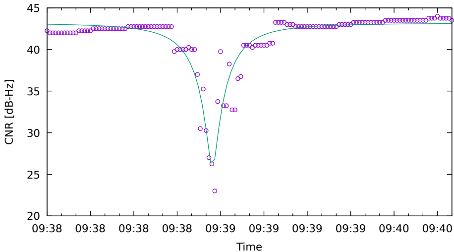
CNR fit for G32 on Xiaomi11T - drive 12 (DOY262)
