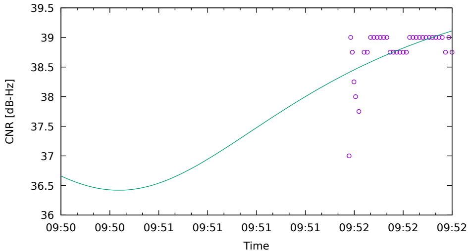
CNR fit for G32 on Xiaomi11T - drive 18 (DOY262)
