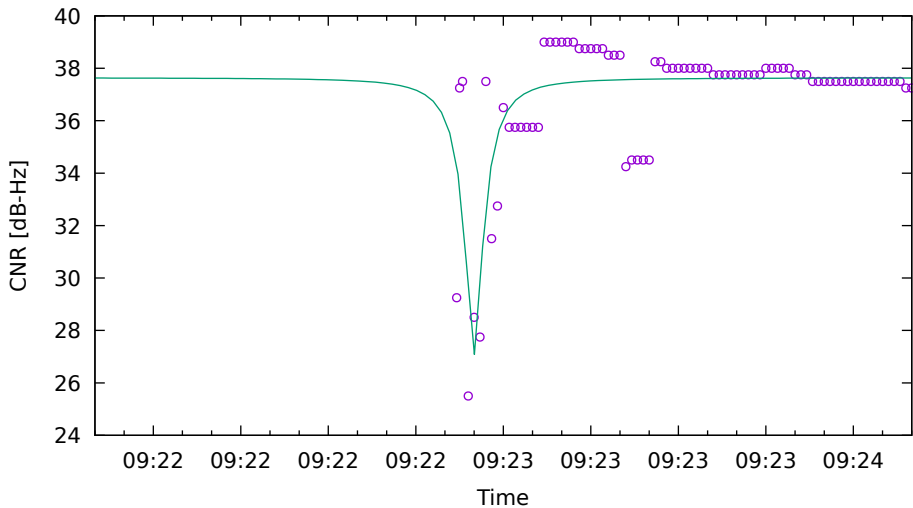
CNR fit for G32 on Xiaomi11T - drive 4 (DOY262)
