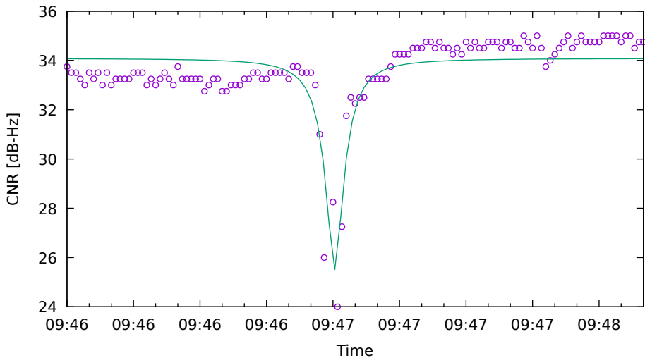
CNR fit for C09 on XiaomiMi8 - drive 16 (DOY262)
