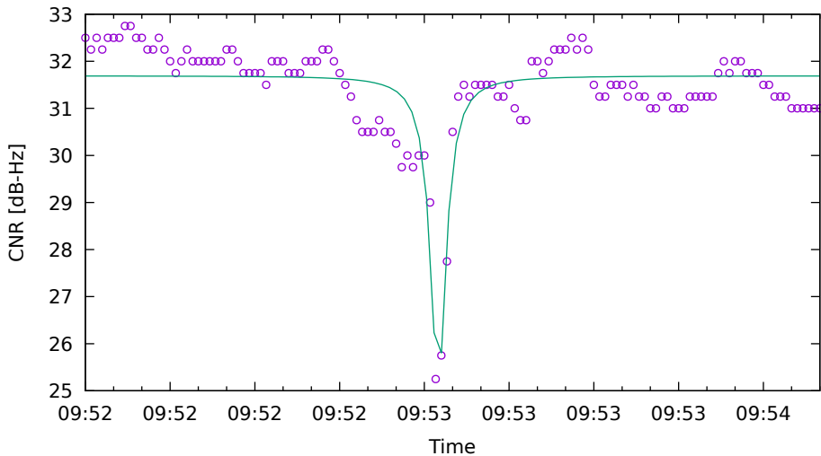
CNR fit for C09 on XiaomiMi8 - drive 19 (DOY262)
