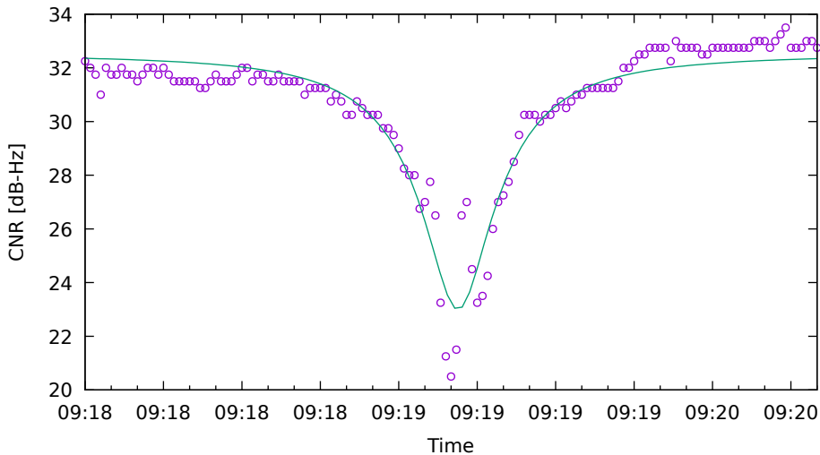
CNR fit for C09 on XiaomiMi8 - drive 2 (DOY262)
