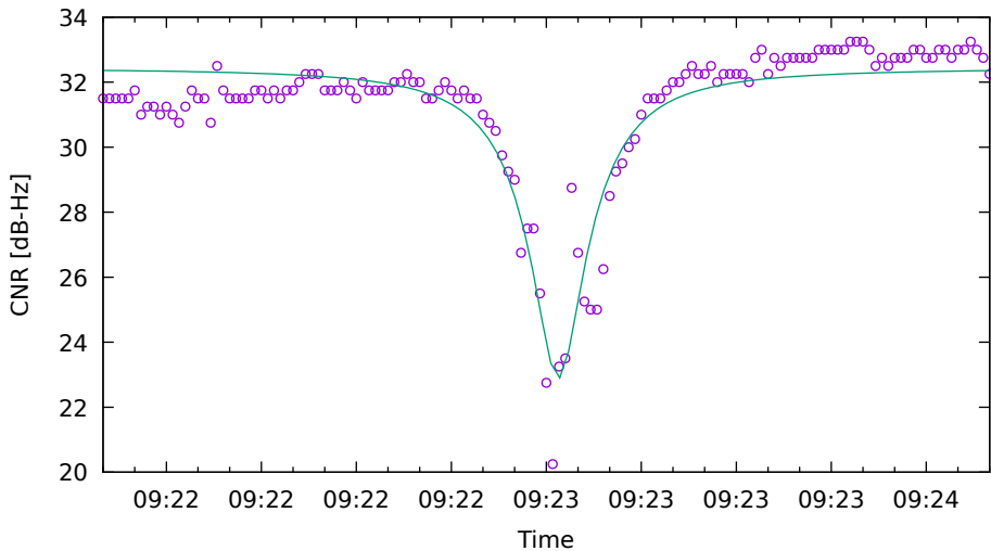
CNR fit for C09 on XiaomiMi8 - drive 4 (DOY262)
