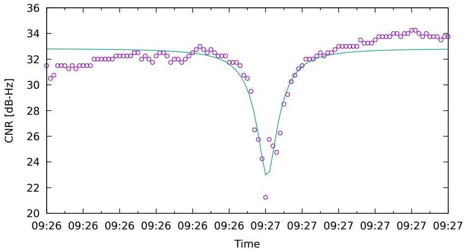
CNR fit for C09 on XiaomiMi8 - drive 6 (DOY262)
