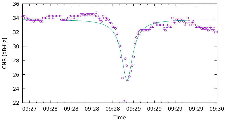
CNR fit for C09 on XiaomiMi8 - drive 7 (DOY262)
