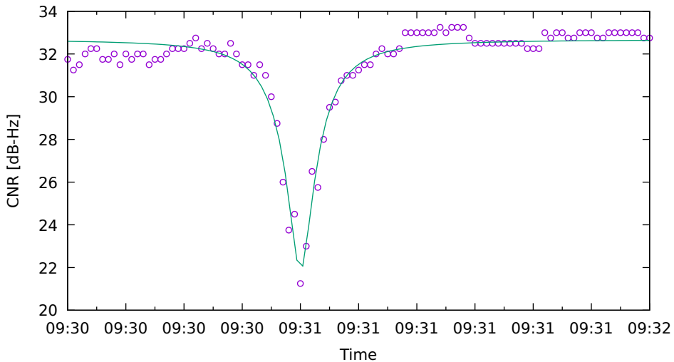
CNR fit for C09 on XiaomiMi8 - drive 8 (DOY262)
