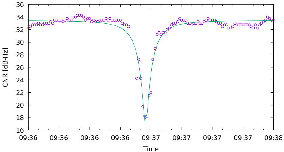
CNR fit for C11 on XiaomiMi8 - drive 11 (DOY262)
