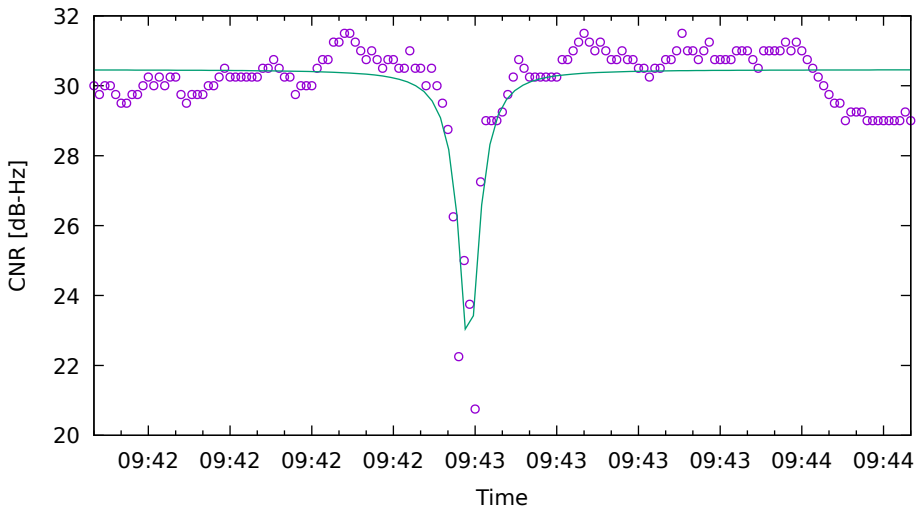
CNR fit for C11 on XiaomiMi8 - drive 14 (DOY262)
