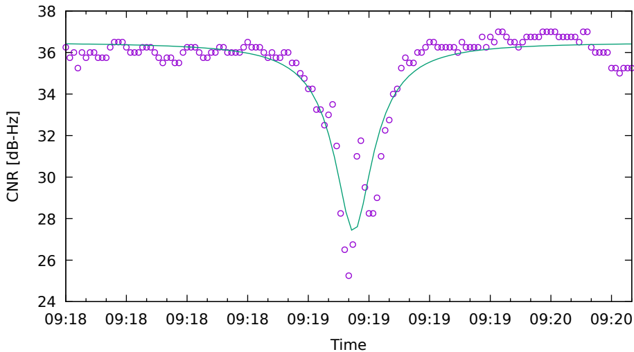
CNR fit for C11 on XiaomiMi8 - drive 2 (DOY262)
